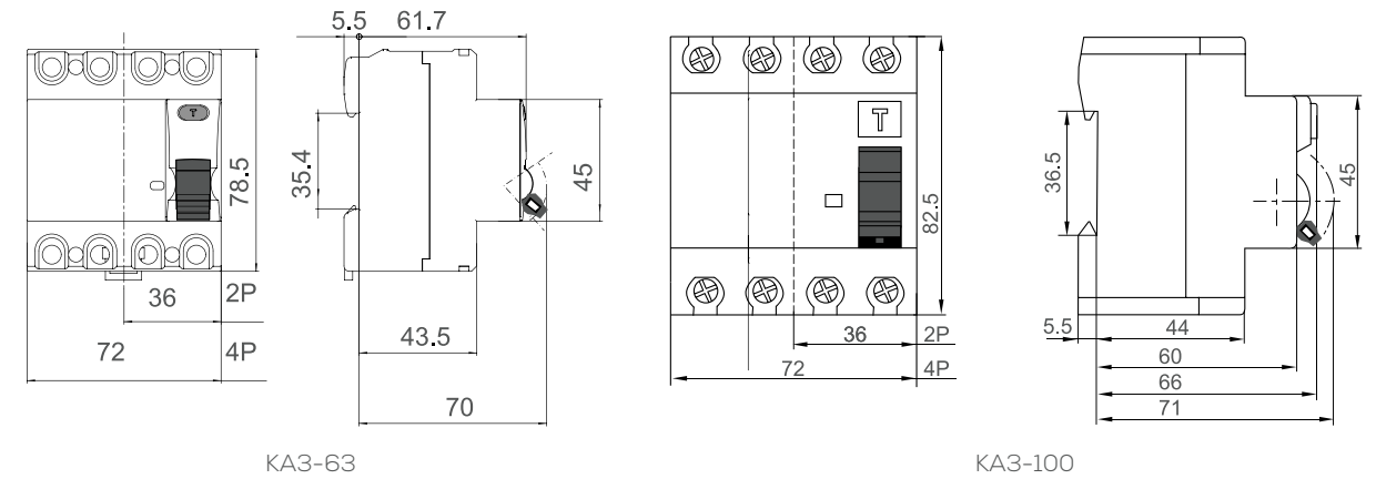
KA3-63
