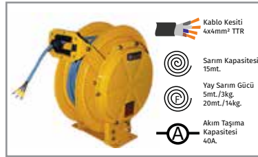
BE0-0003-0315 Kutu 1 Ad.
